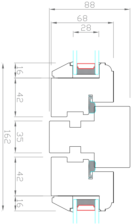
Construction Mullion
