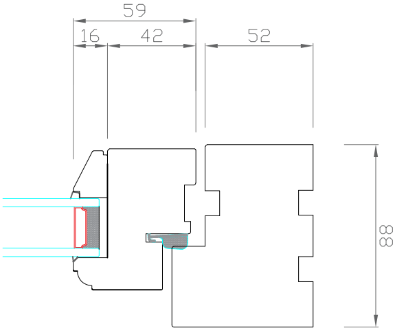
Vertical cross section
