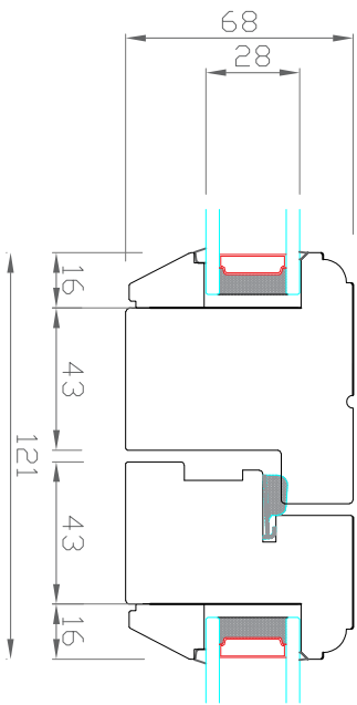
Floating Mullion
