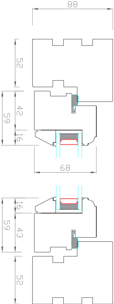
Horizontal cross section
